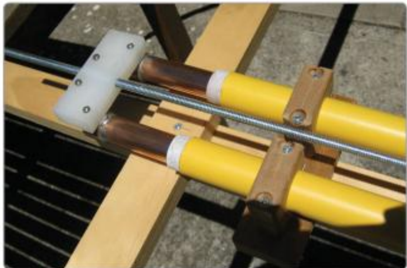
Photo 4: Close up of the timber clamps.
